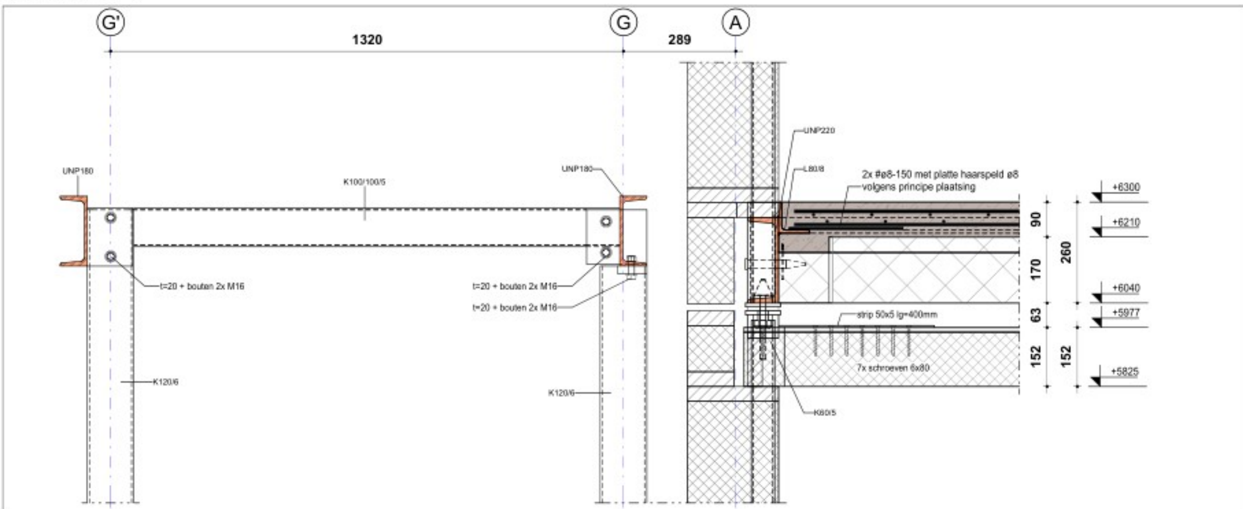
detail 2.01
